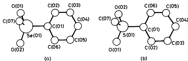
Figure 1. A comparison of bond lengths (Å) and angles (°) in (a) methyl phenyl selenone (X = Se) and (b) (in parentheses) methyl phenyl sulphone (X = S, ref. 22). X–C(01) 1.927(7) (1.832), X–O(01) 1.613(5) (1.453), X–O(02) 1.611(5) (1.465), X–C(07) 1.899(8) (1.761); C(01)–X–O(02) 108.4(3) (106.1), C(01)–X–C(07) 108.1(3) (112.6), C(01)–X–O(01) 107.7(3) (109.9), O(02)–X–C(07) 109.3(3) (107.7), O(02)–X–O(01) 115.2(3) (117.0), C(07)–X–O(01) 107.9(3) (103.8).
